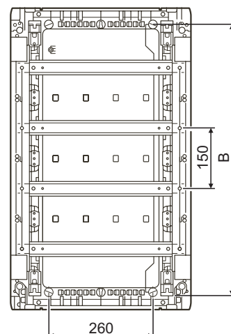
Fixing centre distances and distance between rails
