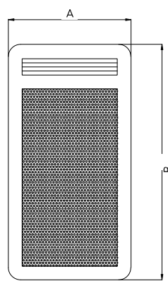
NEF VERTICAL
