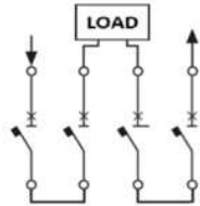
4 poles in series
