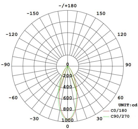
Diagram for RATR6P03038-01 1 in 3000K. Other diagrams available on request
