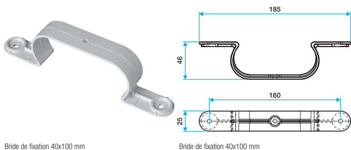
Bride de fixation 40x100 mm
