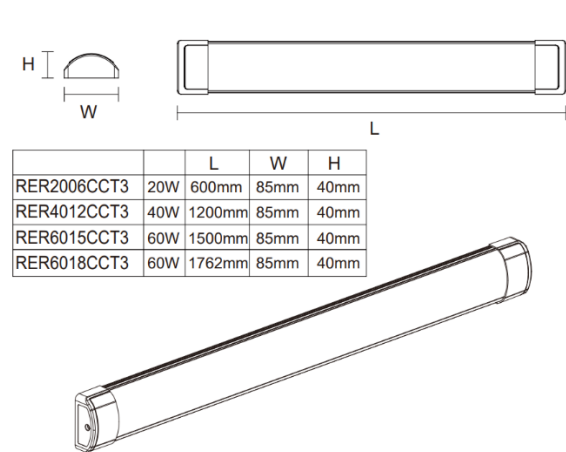
Dimension Diagram
