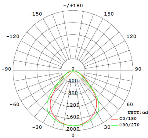
Diagram for RHR40CCT3-10 in 3000K. Other diagrams available on request
