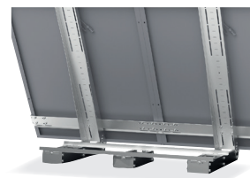
SUPPORT DALLE BÉTON Ref 2679
