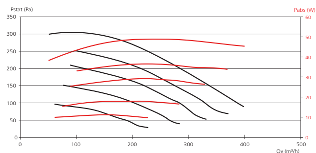
Copernic H 400
