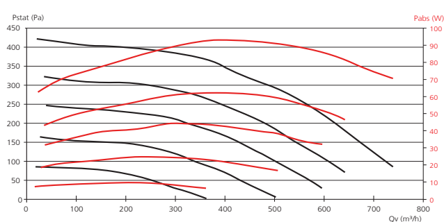
Copernic H 700
