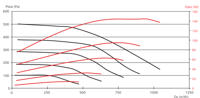
Copernic H 1000
