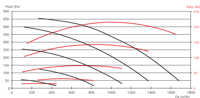
Copernic H 1500
