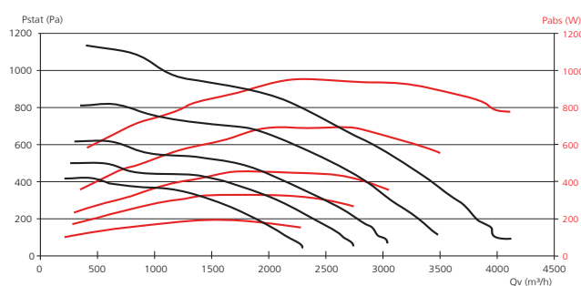
Copernic H 3500
