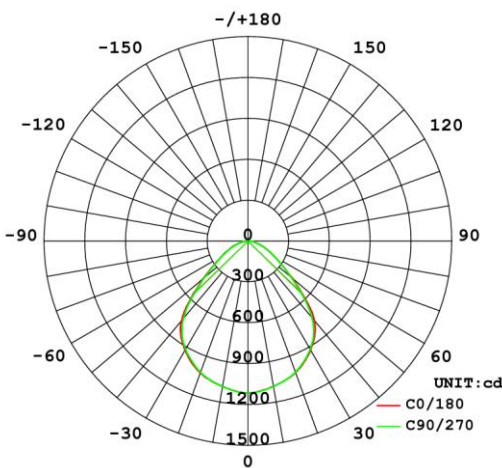
Diagram for RSCX4015-01 in 31W. Other diagrams available on request
