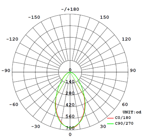
Diagram for RULX-01 in 7W, 4000K. Other diagrams available on request
