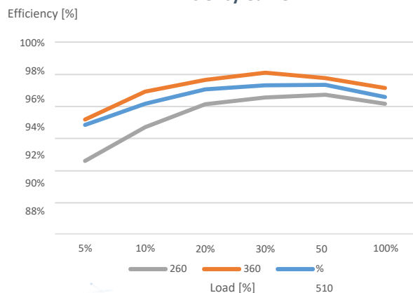
Efficiency Curve
