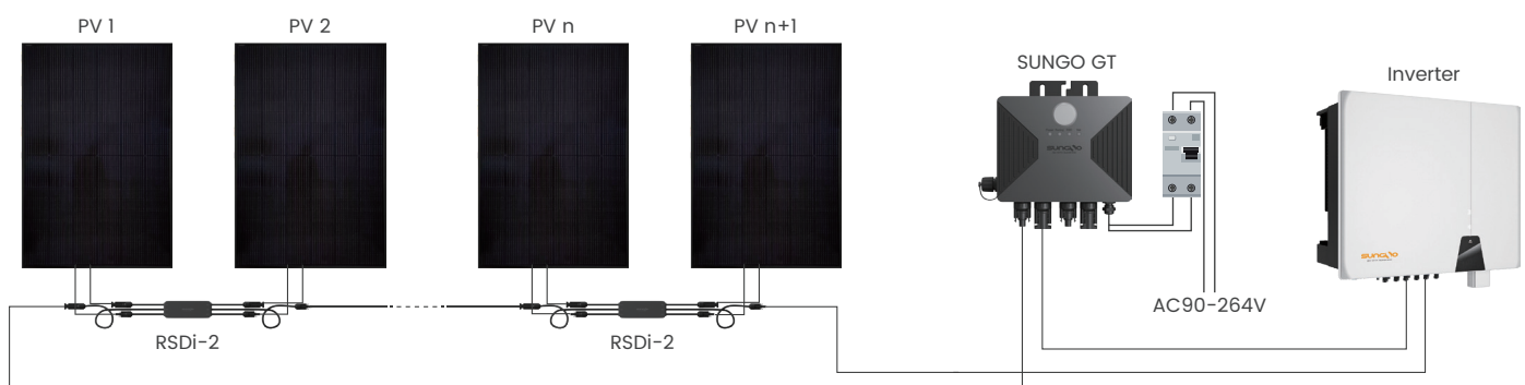
Connection Diagram
