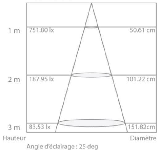
Courbe lux - distance
